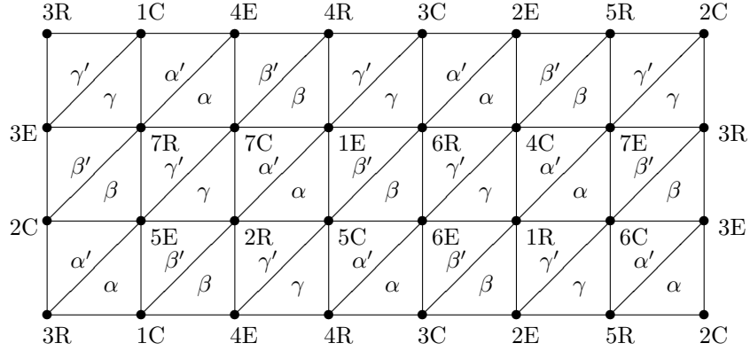
Figure 4: The triangulation T(3, 1, 7) .
