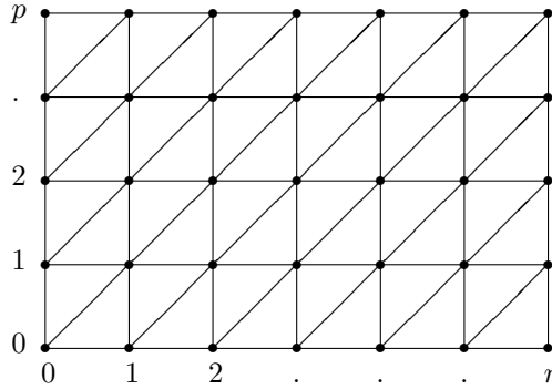
Figure 2: Triangulation of \{(x, y) \in \mathbb{R}^2 : 0 \leq x \leq r, 0 \leq y \leq p\} .
