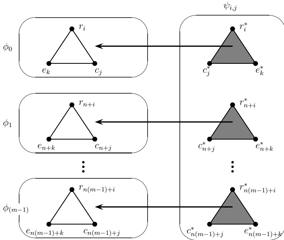
Each \phi_u is an embedding of K_{n,n,n} and \psi_{i,j} is an embedding of K_{m,m,m} .
