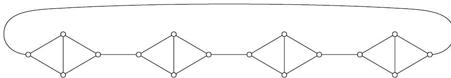
Figure 1: The graph H_{16} .
