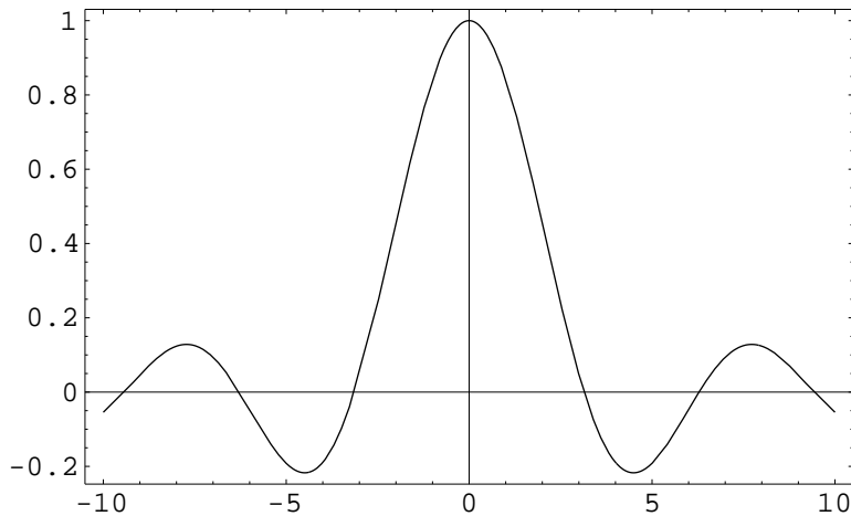
FIG. 2.1. Graph of the function \sin(x)/x .
